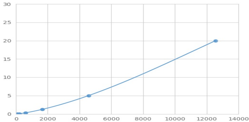
Typical Standard Curve for RPS6Ka1 Magnetic Luminex Assay.
