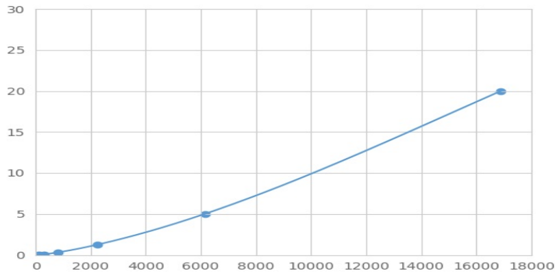
Typical Standard Curve for S100A15 Magnetic Luminex Assay.
