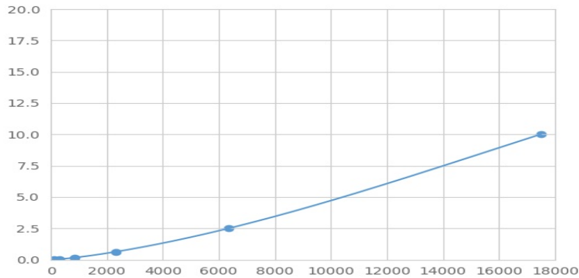
Typical Standard Curve for S100A8 Magnetic Luminex Assay.
