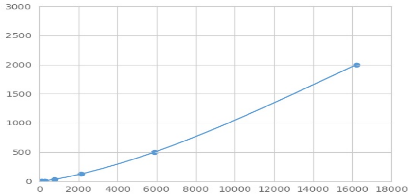
Typical Standard Curve for SLC Magnetic Luminex Assay.
