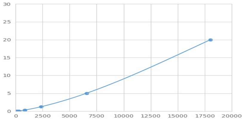
Typical Standard Curve for SQSTM1 Magnetic Luminex Assay.
