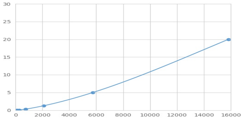
Typical Standard Curve for SPINK5 Magnetic Luminex Assay.
