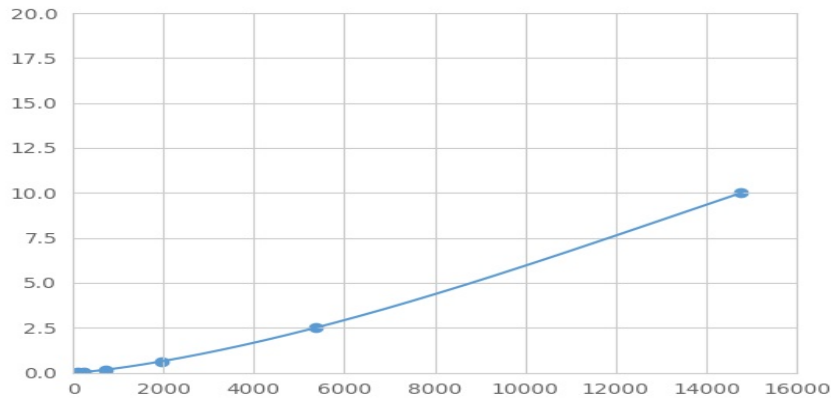
Typical Standard Curve for NIS Magnetic Luminex Assay.
