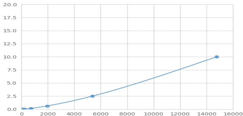
Typical Standard Curve for SMN2 Magnetic Luminex Assay.
