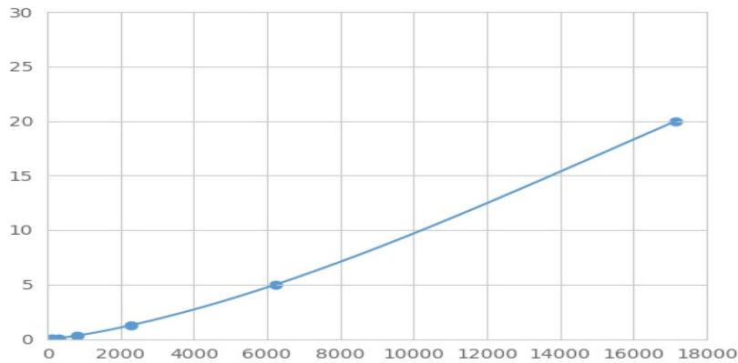
Typical Standard Curve for SYT17 Magnetic Luminex Assay.
