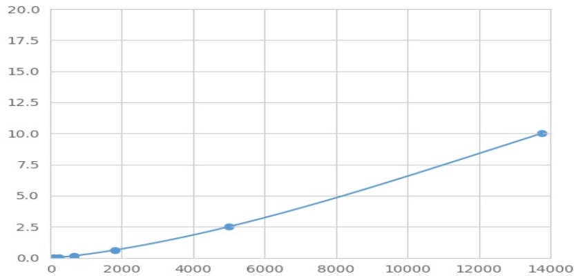
Typical Standard Curve for TBX3 Magnetic Luminex Assay.
