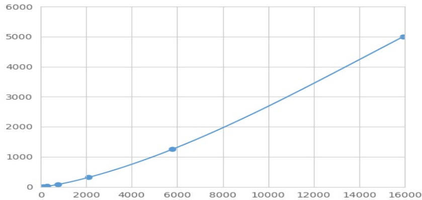
Typical Standard Curve for TDGF1 Magnetic Luminex Assay.
