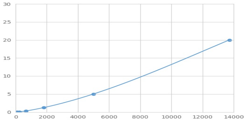
Typical Standard Curve for TrxR2 Magnetic Luminex Assay.
