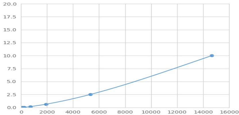
Typical Standard Curve for TLR7 Magnetic Luminex Assay.
