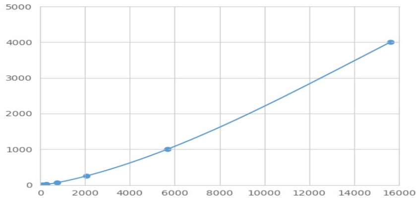
Typical Standard Curve for TICAM1 Magnetic Luminex Assay.
