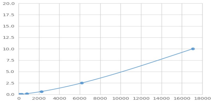
Typical Standard Curve for TCF7L2 Magnetic Luminex Assay.
