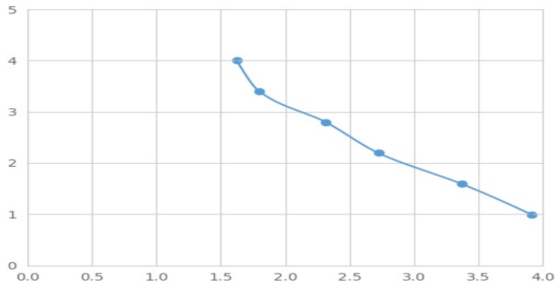
Typical Standard Curve for T3 Magnetic Luminex Assay.
