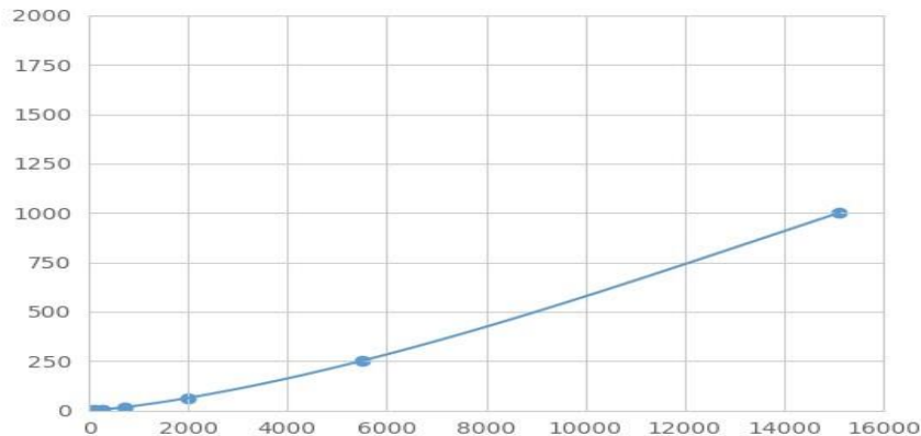
Typical Standard Curve for TNI Magnetic Luminex Assay.
