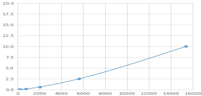
Typical Standard Curve for TRAIL Magnetic Luminex Assay.
