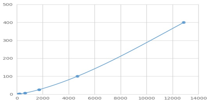
Typical Standard Curve for P53 Magnetic Luminex Assay.
