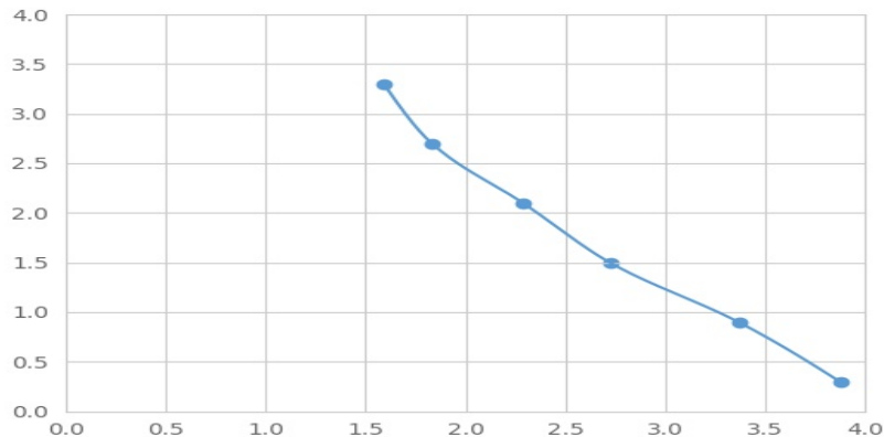
Typical Standard Curve for UCN3 Magnetic Luminex Assay.
