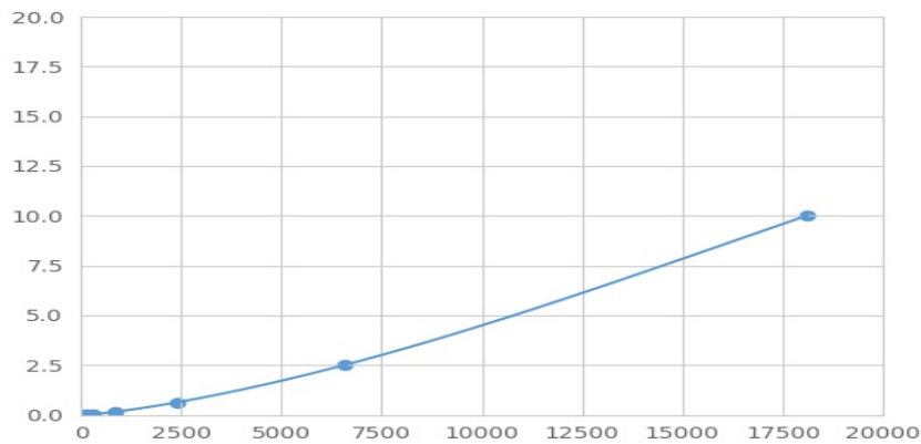
Typical Standard Curve for RELA Magnetic Luminex Assay.
