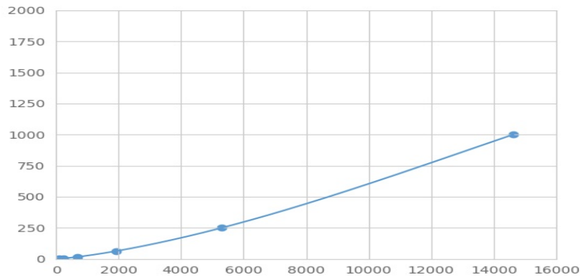
Typical Standard Curve for VEGF165 Magnetic Luminex Assay.
