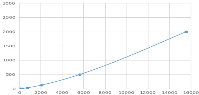
Typical Standard Curve for WNT7A Magnetic Luminex Assay.
