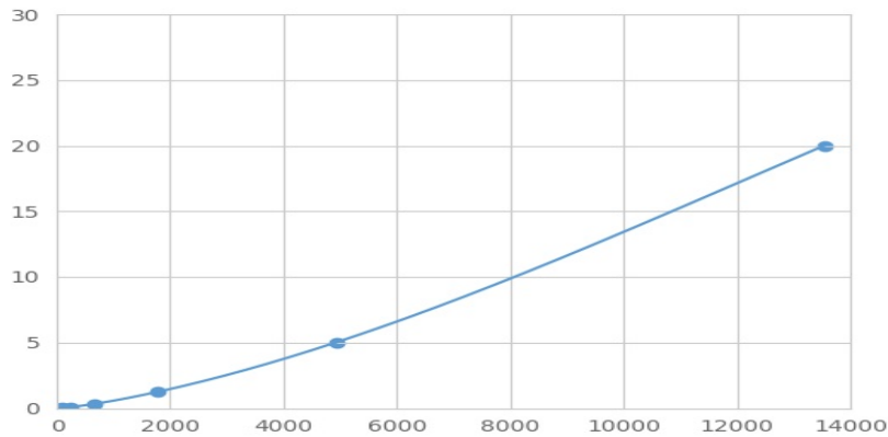
Typical Standard Curve for ZP2 Magnetic Luminex Assay.
