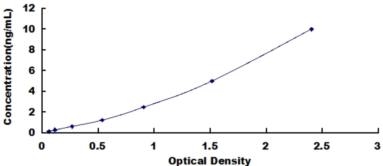
Typical Standard Curve for Adiponectin, Mouse ELISA.
