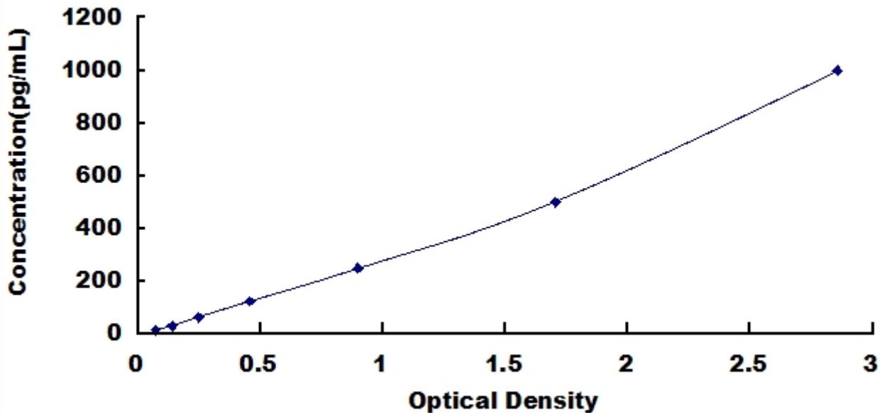
Typical Standard Curve for MCSF, Mouse ELISA.
