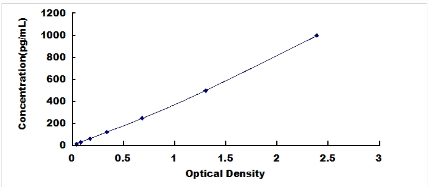
Typical Standard Curve for IL29, Mouse ELISA.
