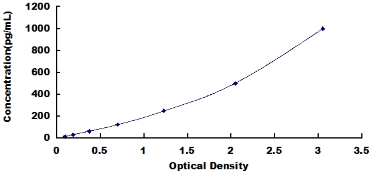
Typical Standard Curve for MCP2, Mouse ELISA.
