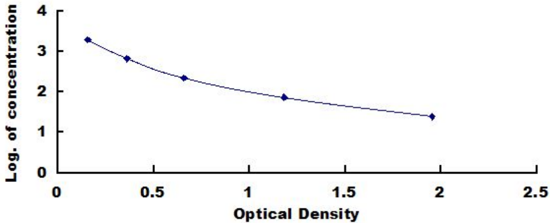
Typical Standard Curve for PP, Rat ELISA.
