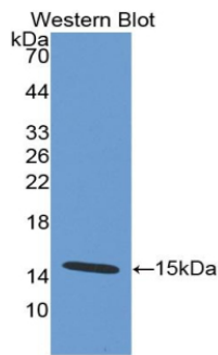
Figure. Western Blot; Sample: Recombinant DEFa5, Human.
