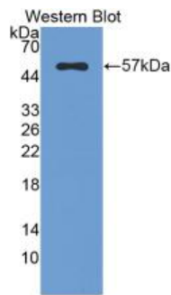
Figure. Western Blot; Sample: Recombinant FGb, Rat.
