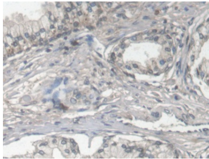
DAB staining on IHC-P; Samples: Human Prostate Tissue; Primary Ab: 30µg/ml Mouse Anti-Human FBLN1 Antibody Second Ab: 2µg/mL HRP-Linked Caprine Anti-Mouse IgG Polyclonal Antibody (Catalog: SAA544Mu19)
