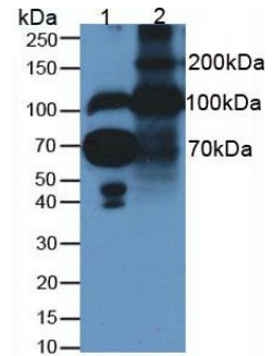
Figure. Western Blot; Samples. Lane1: Human Serum; Lane2: Rat Placenta Tissue;
