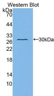
Figure. Western Blot; Sample: Recombinant FBLN1, Human.
