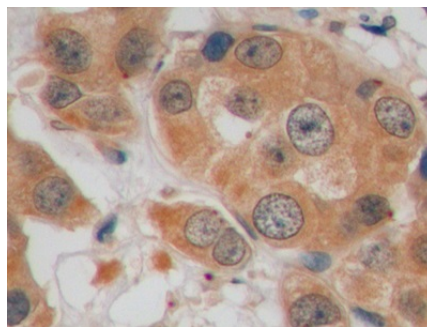
DAB staining on IHC-P; Sample: Human Breast cancer Tissue; Primary Ab: 10µg/ml Mouse Anti-Human GLUT1 Antibody Second Ab: 2µg/mL HRP-Linked Caprine Anti-Mouse IgG Polyclonal Antibody (Catalog: SAA544Mu19)
