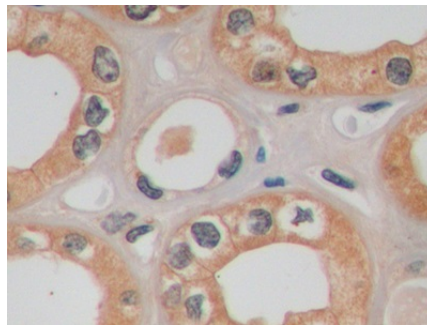
DAB staining on IHC-P; Sample: Human Kidney Tissue; Primary Ab: 10µg/ml Mouse Anti-Human GLUT1 Antibody Second Ab: 2µg/mL HRP-Linked Caprine Anti-Mouse IgG Polyclonal Antibody (Catalog: SAA544Mu19)
