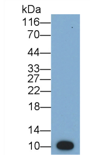
Figure. Western Blot; Sample: Recombinant GLUT1, Human.
