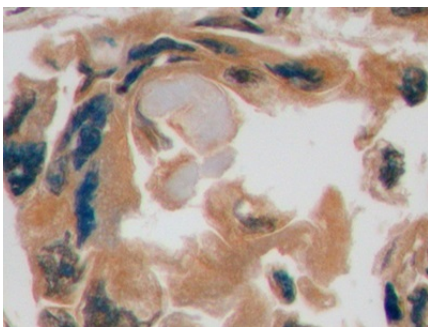
DAB staining on IHC-P; Sample: Human Lung cancer Tissue; Primary Ab: 10µg/ml Mouse Anti-Human GLUT1 Antibody Second Ab: 2µg/mL HRP-Linked Caprine Anti-Mouse IgG Polyclonal Antibody (Catalog: SAA544Mu19)
