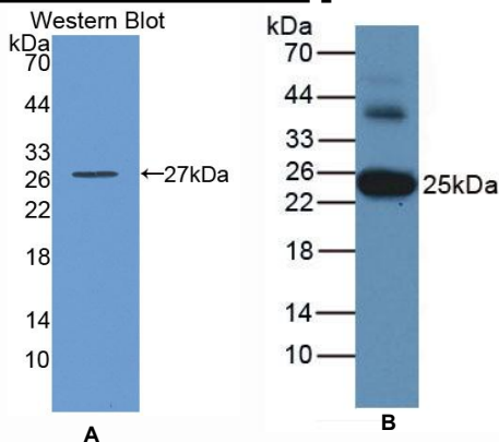
Figure 1. Western Blot
