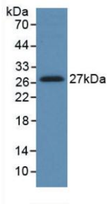
Figure. Western Blot; Sample: Recombinant HGF, Human.
