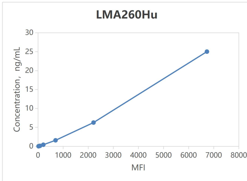
Typical Standard Curve for Multiplex Assay Kit.
