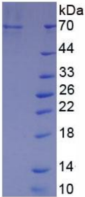
Figure 1. SDS-PAGE
