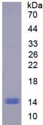
Figure 1. SDS-PAGE
