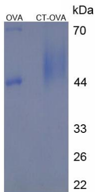
Figure 1. SDS-PAGE of OVA Conjugated CT
