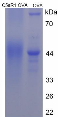
Figure 2. SDS-PAGE of OVA Conjugated C5aR1
