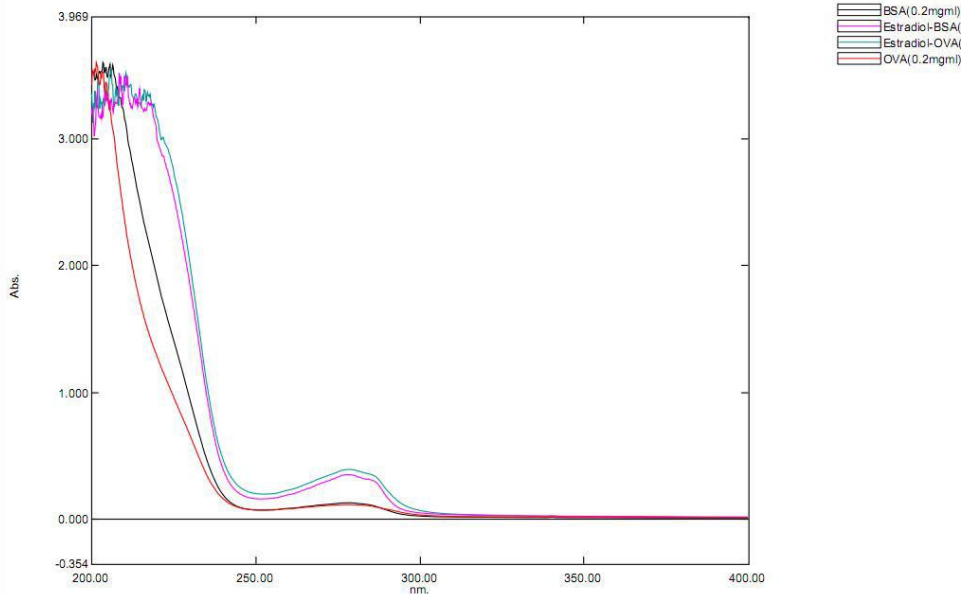
Figure 2. UV-spectrum
