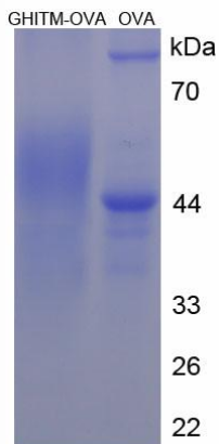
Figure 2. SDS-PAGE of OVA Conjugated GHITM
