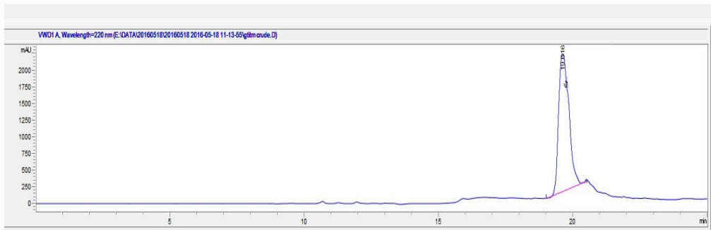
Figure 1. HPLC of the Original Peptide
