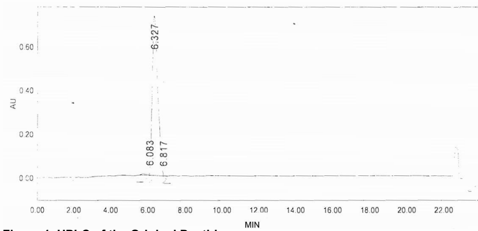
Figure 1. HPLC of the Original Peptide
