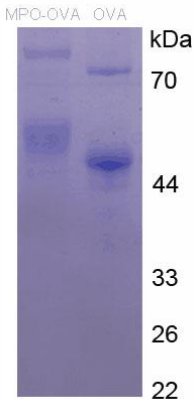
Figure 2. SDS-PAGE of OVA Conjugated MPO
