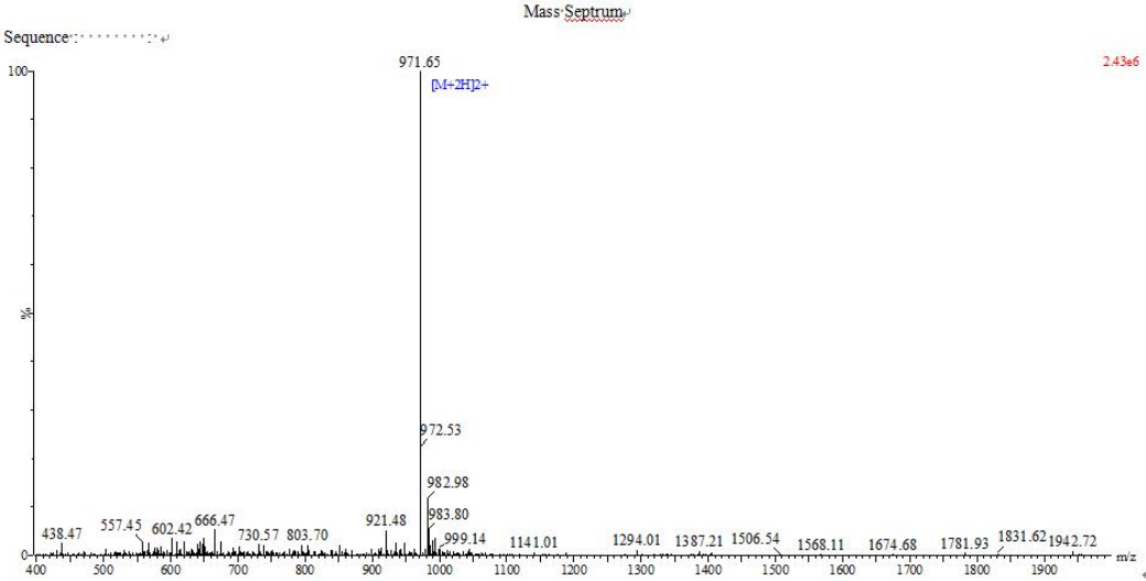
Figure 1. MASS Spectrometry of the Original Peptide
