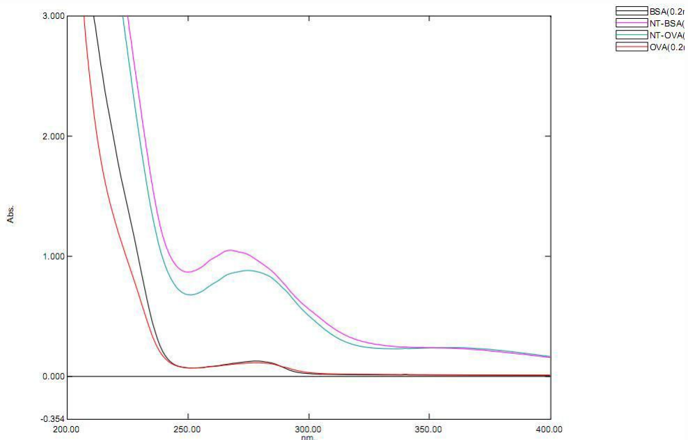
Figure 2. UV-spectrum
