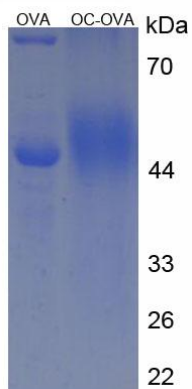
Figure 3. SDS-PAGE of OVA Conjugated OC
