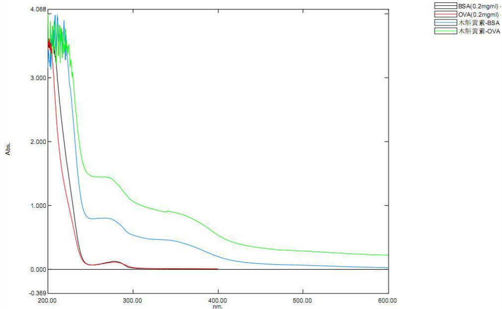
Figure 1. UV-spectrum
