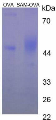
Figure 1. SDS-PAGE
