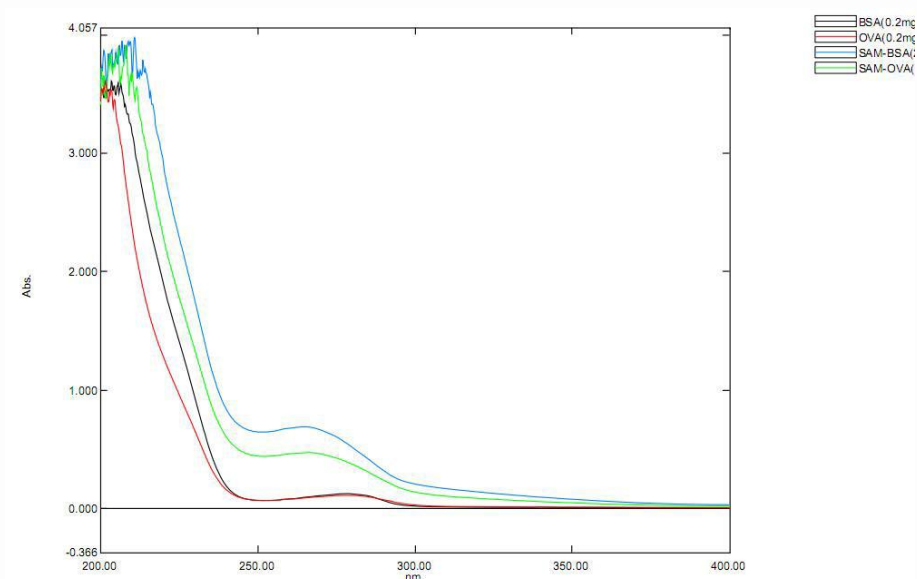
Figure 2. UV-spectrum
