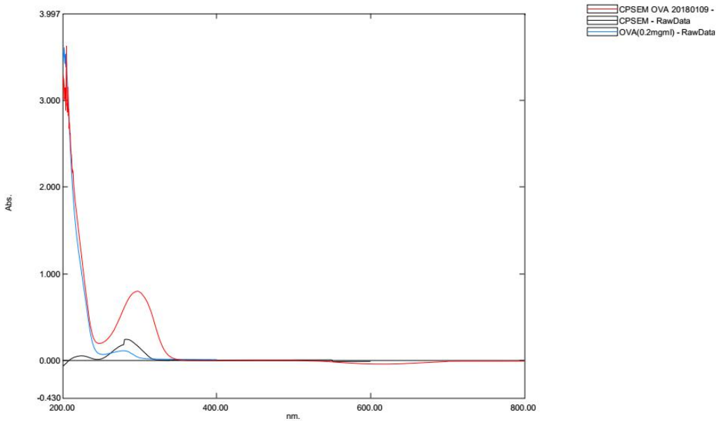
Figure 2. UV-spectrum
