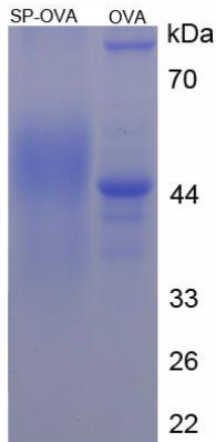
Figure 1. SDS-PAGE of OVA Conjugated SP
